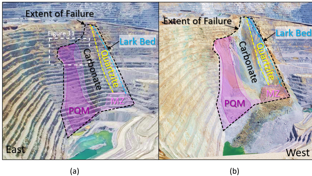
Figure 2 (a) Photograph of the pit slope prior to the Leo Failure with generalised contacts for the lithologic units within the failure boundary; (b) Photograph of the post-failure slope with generalised key lithologic units within the failure boundary
