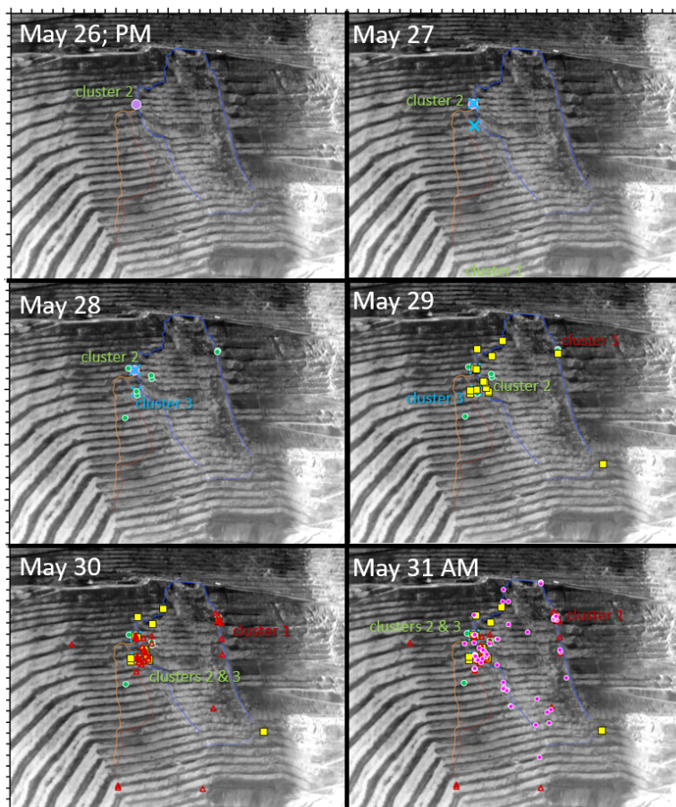
Figure 6 Still image at 7:30 am on 31 May from thermal video with day-to-day addition of positions of rockfall origins for each day leading up the Leo Failure. The image is the same for each day shown
