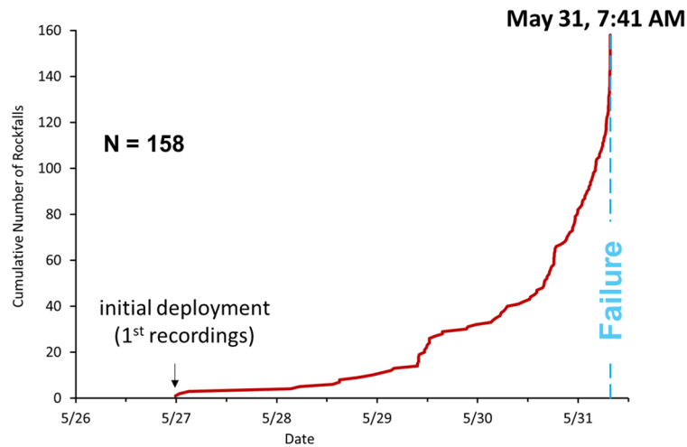
Figure 5 Plot of cumulative rockfalls versus time leading up to the Leo Failure
